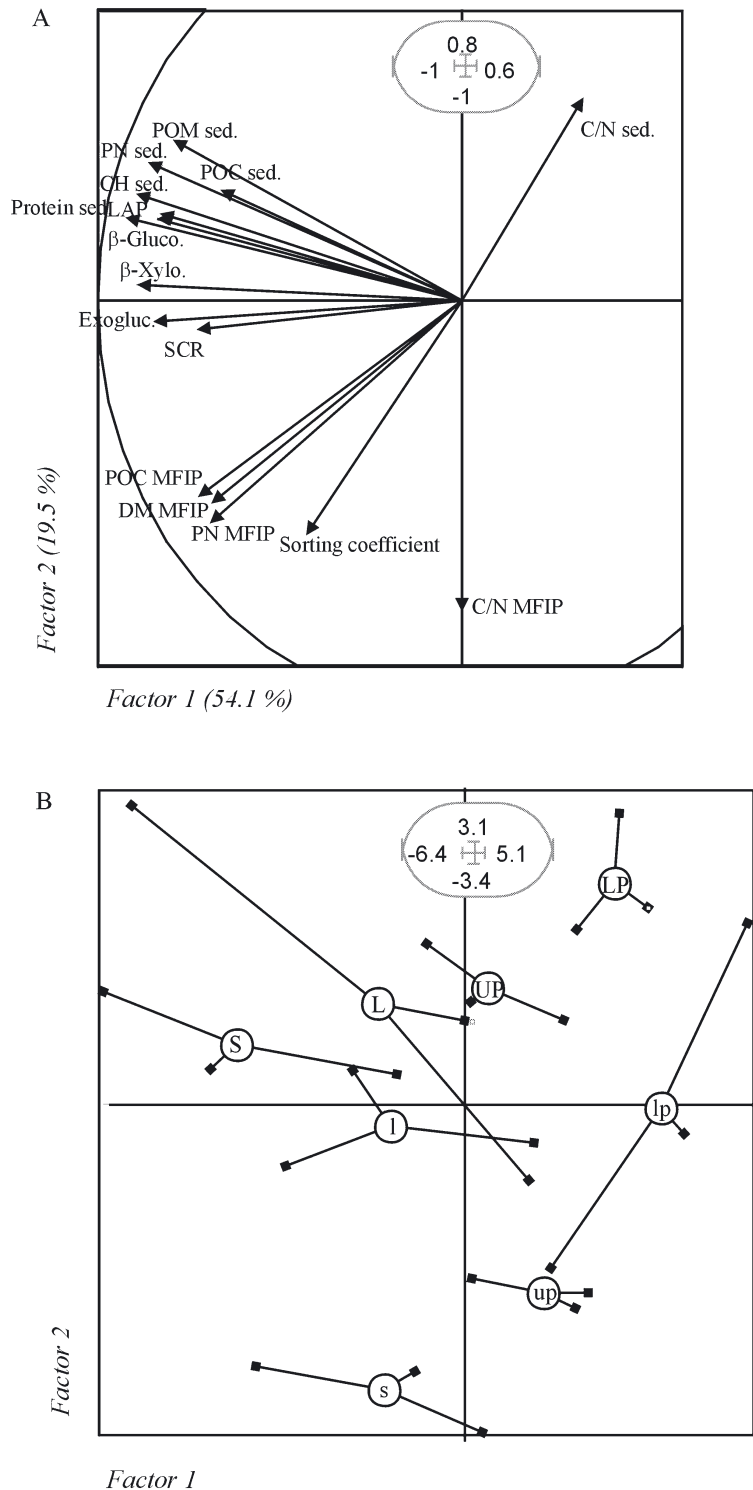
Fig. 6. (A) PCA ordination plot of bacterial and environmental variables. (B) Factorial map of different zones of subaqueous dune for the 2 sampling months. S: stoss side (September), UP: upper plateau (September); LP: lower plateau (September); L: lee side (September); s: stoss side (November); up: upper plateau (November); lp: lower plateau (November); l: lee side (November). Other abbreviations as in Figs. 3–5
