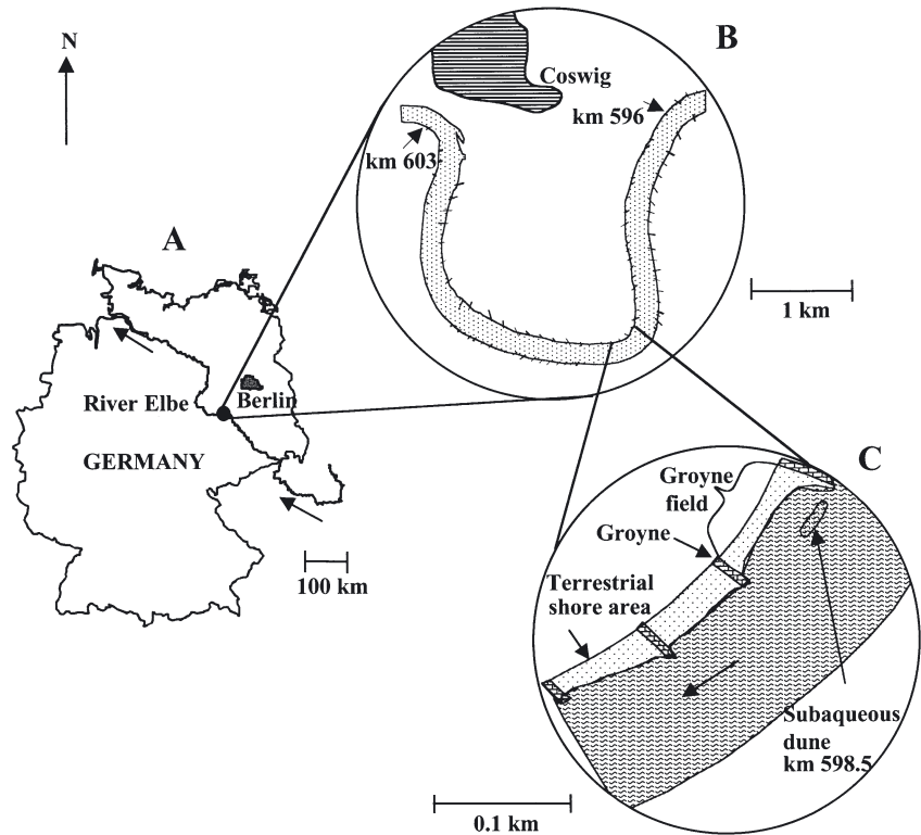
Fig. 1. Location of study site: (A) Map of Germany showing River Elbe. (B) Investigated river reach near Coswig town; km = river kilometres counted from source; whiskers along river margin = groynes. (C) Subaqueous dune and 3 groyne fields investigated at the sampling site
