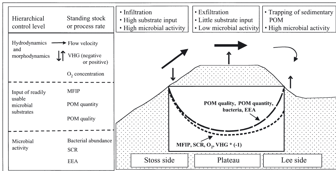
Fig. 7. Schematic model of spatial patterns of hydrodynamics, morphodynamics, fine particles, particulate organic matter and microbial activity within subaqueous dune. Direction and relative level of the variables are represented by direction and relative size of arrows and by relative extension of line (in similarity to the percentage increase) compared to plateau site, respectively, EEA: extracellular enzyme activities; MFIP: mobile fine interstitial particles; POM quantity: total particulate organic matter content; POM quality: sedimentary content of carbohydrates, protein, phaeopigments; SCR: sediment community respiration; VHG: vertical hydraulic gradient
