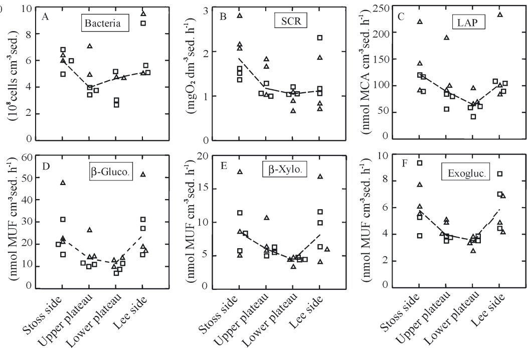
Fig. 5. Characteristics of bacterial variables along transect of the 3 morphodynamic zones of the subaqueous dune in September and November 2000. Data of plateau are shown separately for upper and lower plateau. (A) Bacterial abundance, (B) sediment community respiration, (C) leucine aminopeptidase, (D) \beta -glucosidase, (E) \beta -xylosidase, and (F) exo-1,4- \beta -glucanase. For each zone, medians are connected by dashed line. MCA: methylcumarinyl; MUF: methylumbelliferyl
