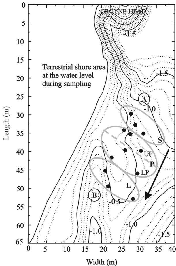
Fig. 2. Contour map showing water depths at study site and sampling positions (●) along transect (A–B) within the 3 morphodynamic zones (stoss, plateau, lee) of subaqueous dune. S: stoss side; P: plateau; UP: upper plateau; LP: lower plateau; L: lee side; arrow indicates flow direction
